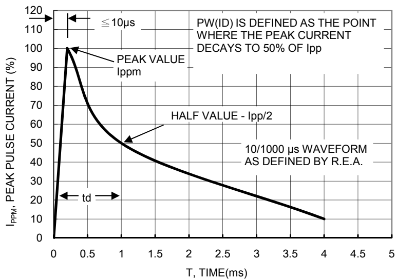
FIG. 11 PULSE WAVEFORM
