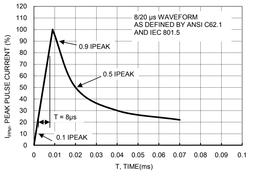
FIG. 12 PULSE WAVEFORM
